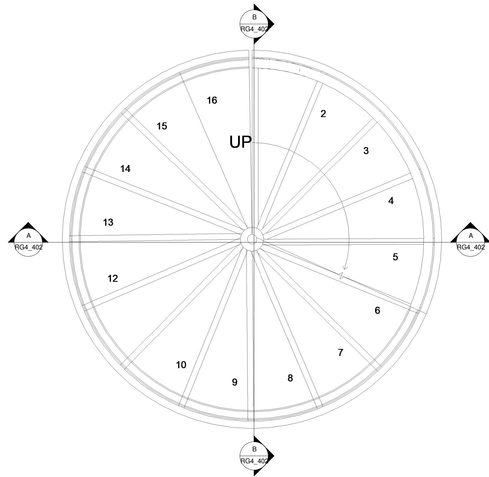
1 DETAIL ROOF STAIRCASE_PLAN 1 : 10
